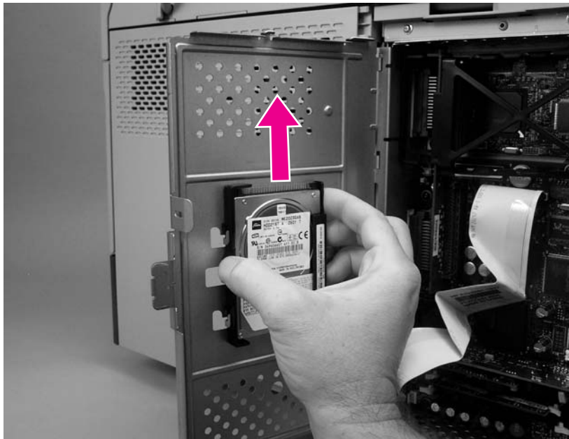
Figure 6-34 Remove the hard drive (2 of 2)
