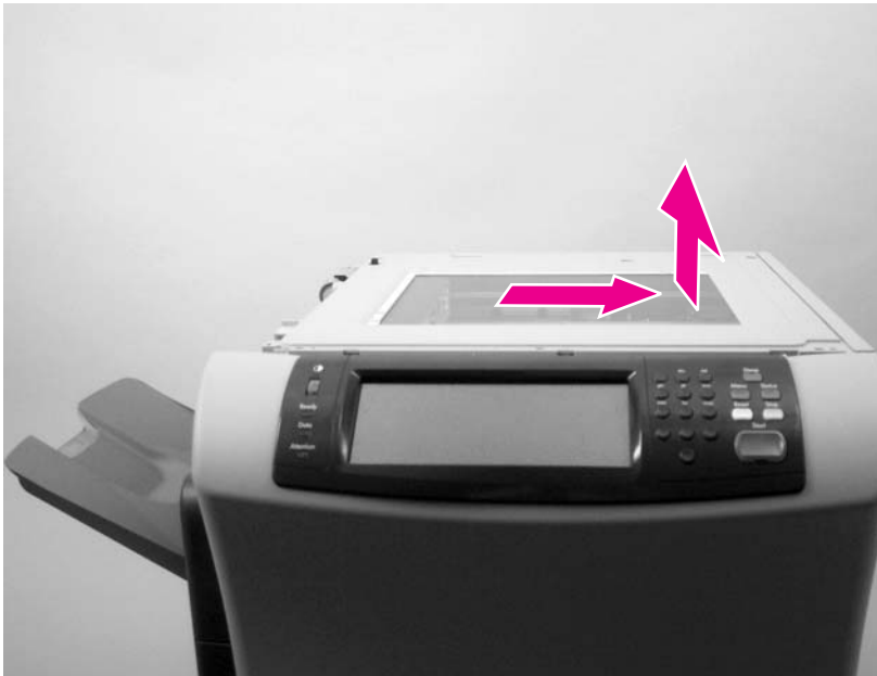
Figure 6-179 Remove the scanner assembly (8 of 8)
