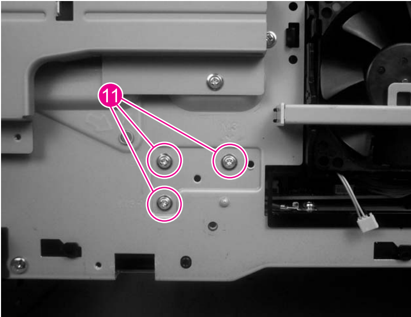
Figure 6-155 Remove the engine power supply (7 of 10)
