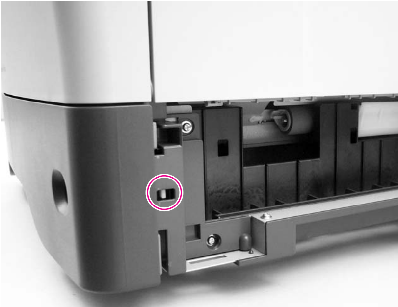
Figure 7-11 Tray 2 jam-access-cover switch, SW105
