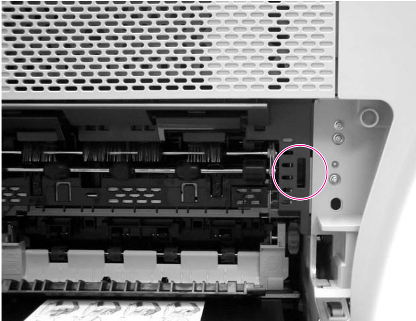
Figure 7-8 Output-bin detection switch, SW103
