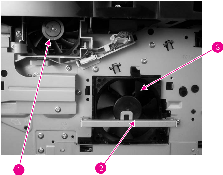
Figure 7-12 Front-side fans
