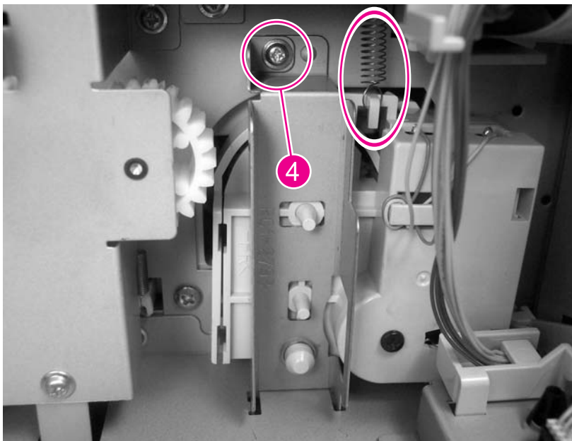
Figure 6-139 Remove the lifter-drive assembly (4 of 5)
