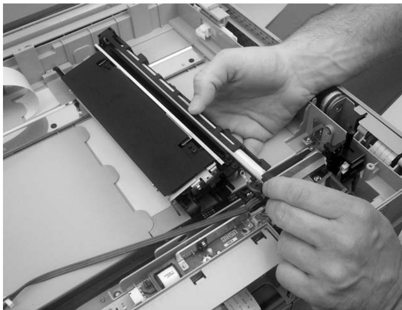
Figure 6-195 Remove the scanner bulb (2 of 2)
