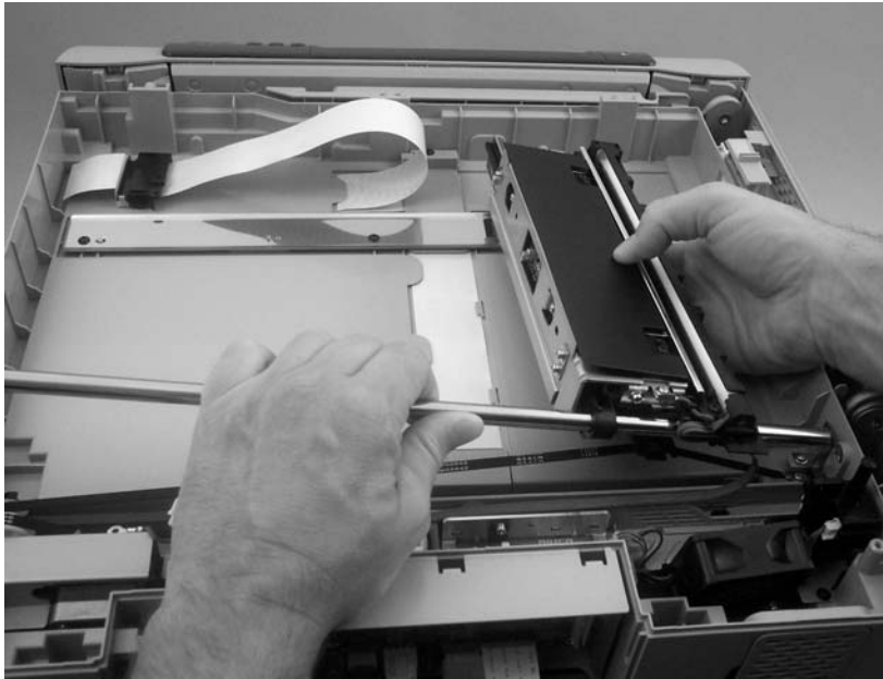
Figure 6-191 Remove the optical unit (5 of 7)
