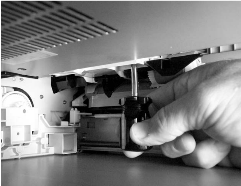
Figure 6-163 Remove the tray 2 paper-present sensor
