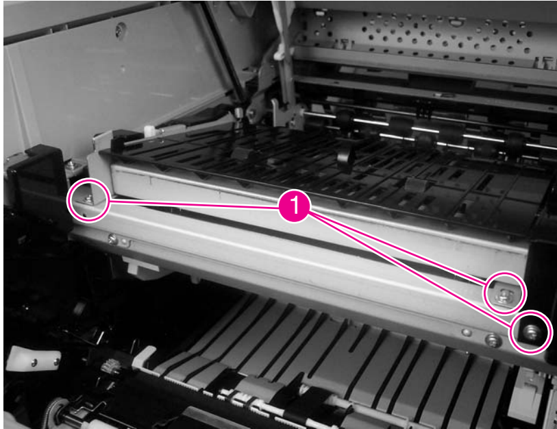
Figure 6-52 Remove the reversing assembly (1 of 8)
