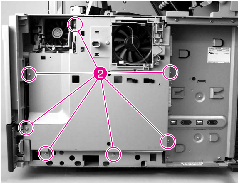
Figure 6-137 Remove the lifter-drive assembly (2 of 5)
