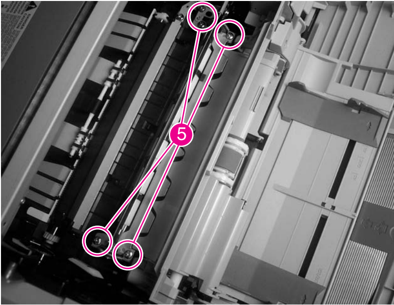
Figure 6-128 Remove the registration assembly (6 of 6)
