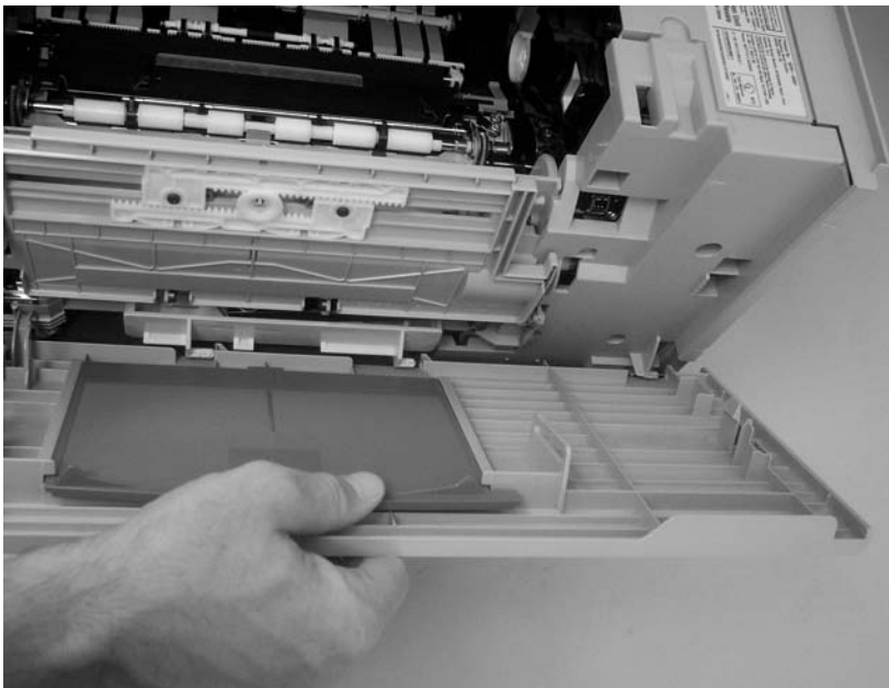
Figure 6-77 Remove the tray 1 assembly (2 of 5)
