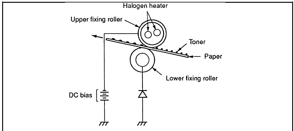
Image Fusing
