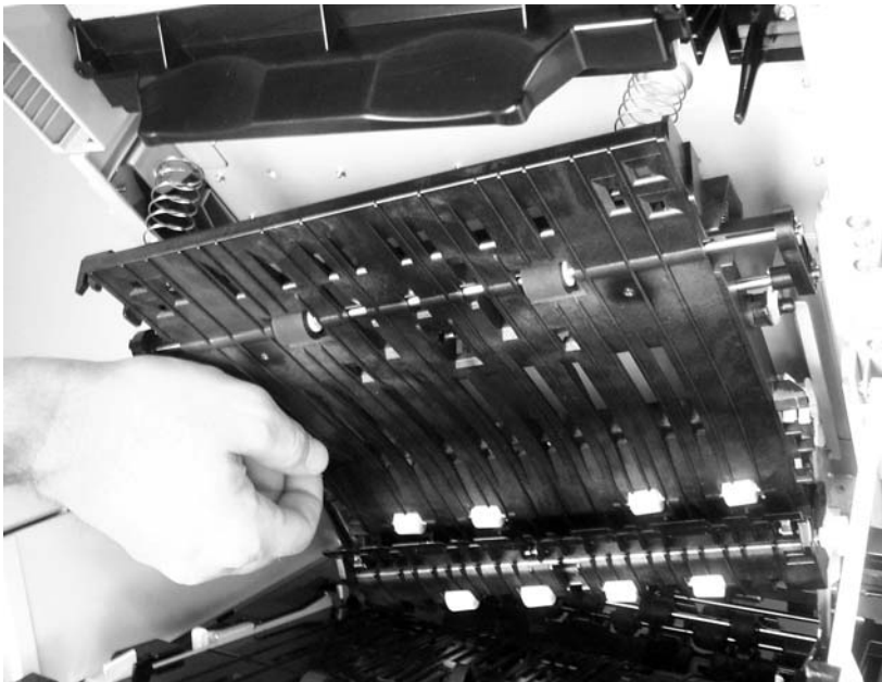
Figure 5-50 Remove the reversing-separation-guide assembly (2 of 2)
