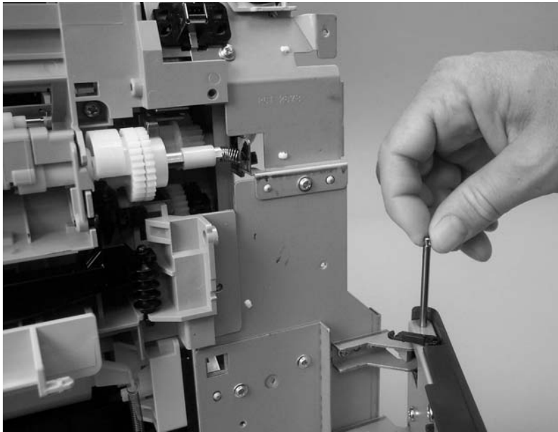
Figure 5-84 Remove the tray 1 feed-assembly (2 of 13)
