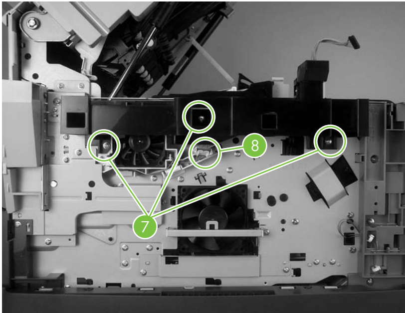
Figure 5-65 Remove the main and reversing-unit fans (7 of 9)
