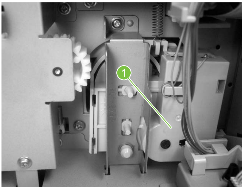
Figure 4-80 Rear-side motors (2 of 2)
